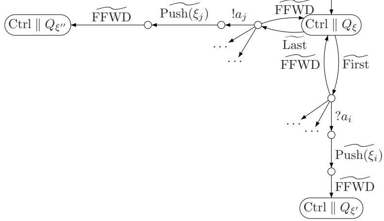
Figure 1: Transition system sketch of the workings of the Ctrl process in parallel with a queue. By \langle equation \rangle we indicate the \tau -steps generated by that equation, up to the point where another process equation is entered.
