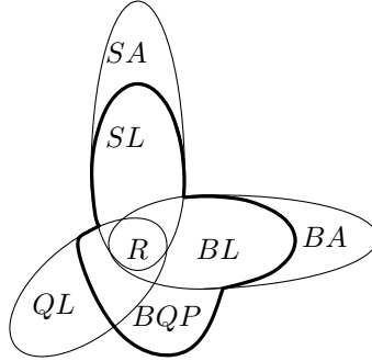
Figure 2: Chomsky hierarchy including expressivity of BQP. S and B stand for stack and bag respectively. A stands for automata, L stands for language. R is the class of regular languages. QL are the queue languages.
